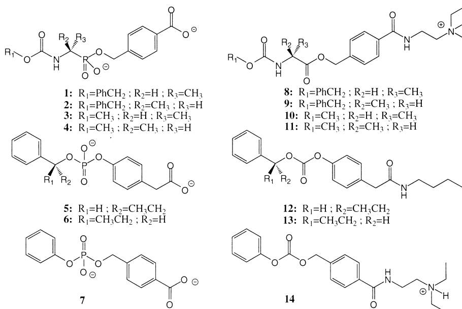
Scheme 1. Structures of haptens 1–7 and substrates 8–14 .
