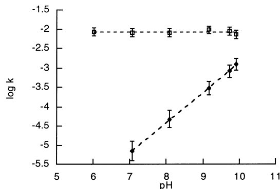
Figure 1. pH Dependence of the hydrolysis reactions of carbonates 22 and 23 . The open squares represents points for carbonate 23 , the darkened diamonds represent points for carbonate 22 . The pH independence of hydrolysis for carbonate 23 was taken as evidence for a mechanism other than \text{B}_{\text{AC}}2 . Substrates 20 and 21 behaved in a manner analogous to 22 , while substrate 24 behaved in a manner analogous to 23 . These were omitted for clarity.
