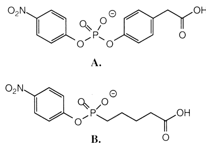
Scheme 3. (A) The structures of the hapten used by Gallacher and Brocklehurst et al. 1–3,5,10,11 to immunize sheep. (B) The structure of the hapten used by Suzuki et al. 7 to immunize rabbits.
