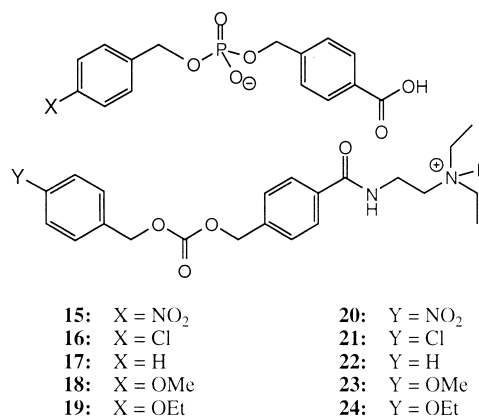
Scheme 2. Structures of haptens 15–19 and substrates 20–24 .
